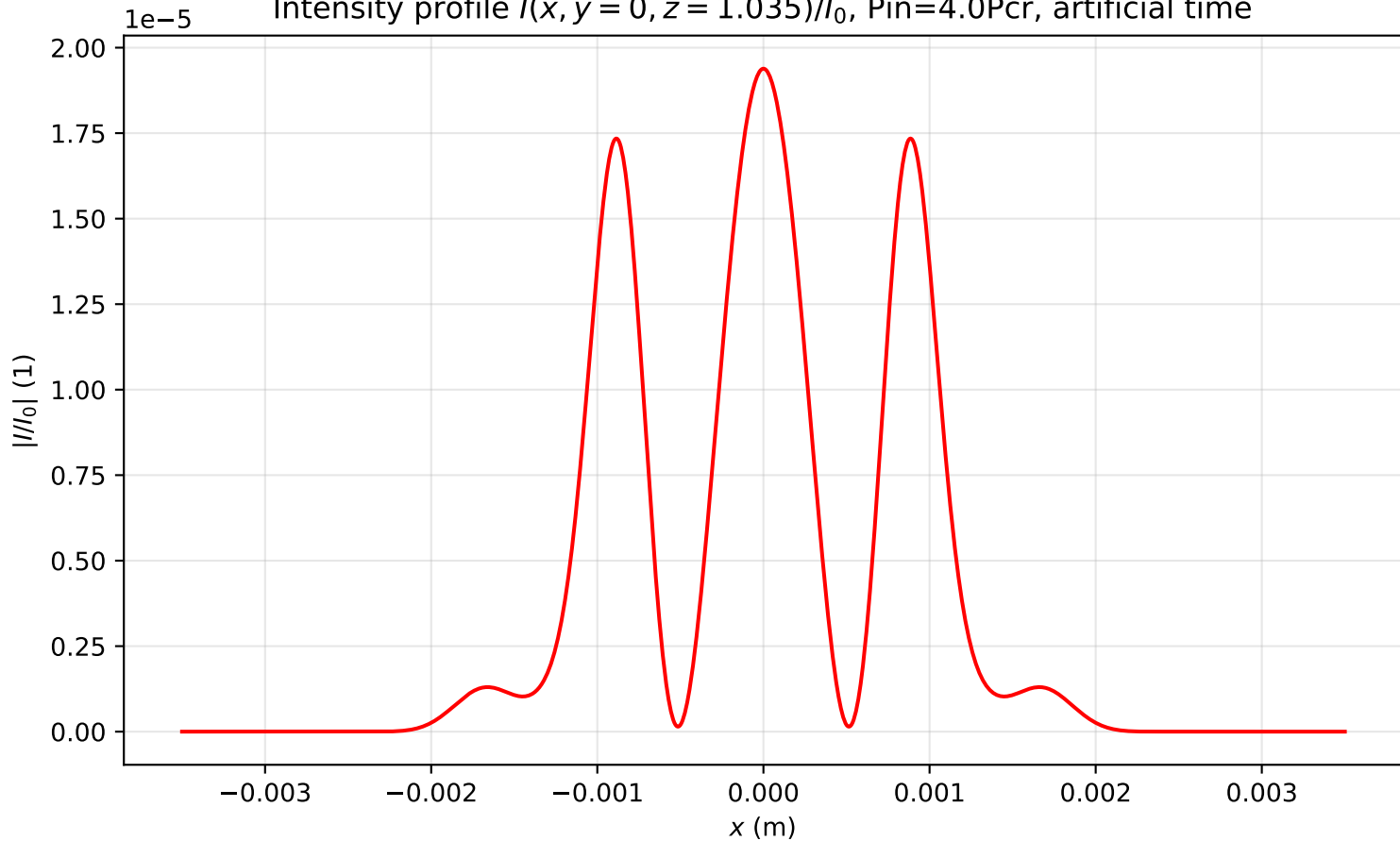
Intensity profile I(x, y = 0, z = 1.035)/I_0 , P_{in}=4.0P_{cr} , artificial time
